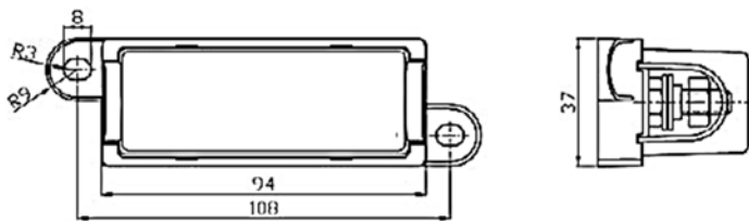
Fuse holder for MEGA fuse
